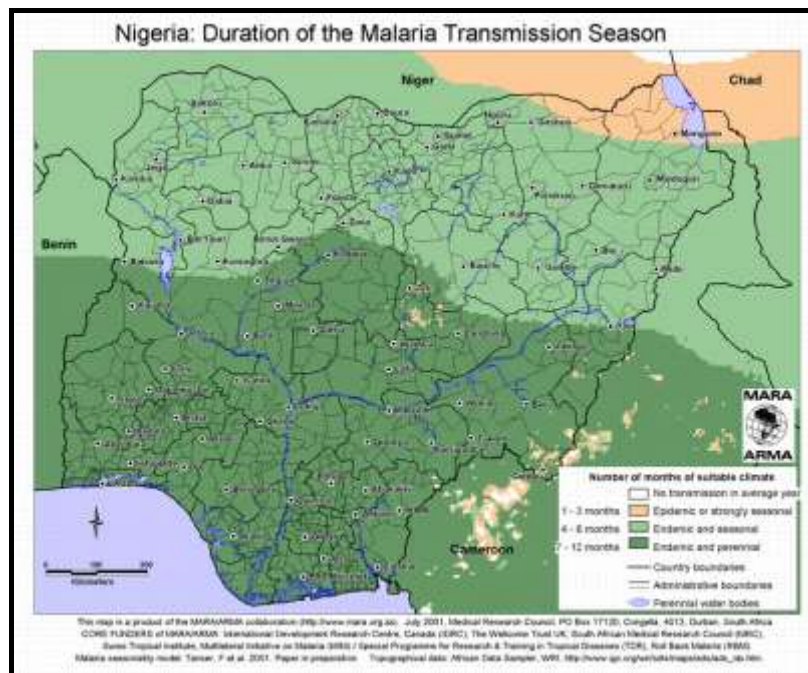
Figure 4: Seasonality of malaria transmission
