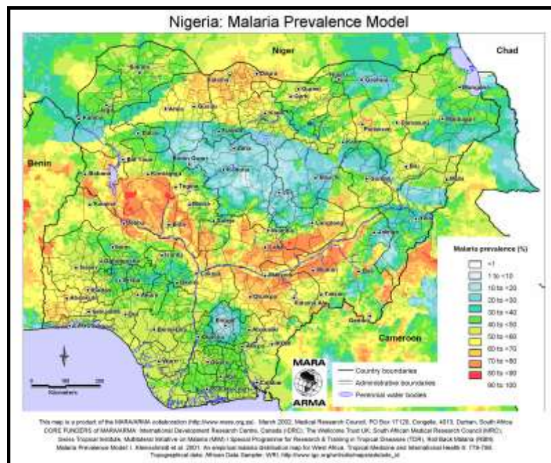
Figure 5: Distribution of projected malaria prevalence rates
