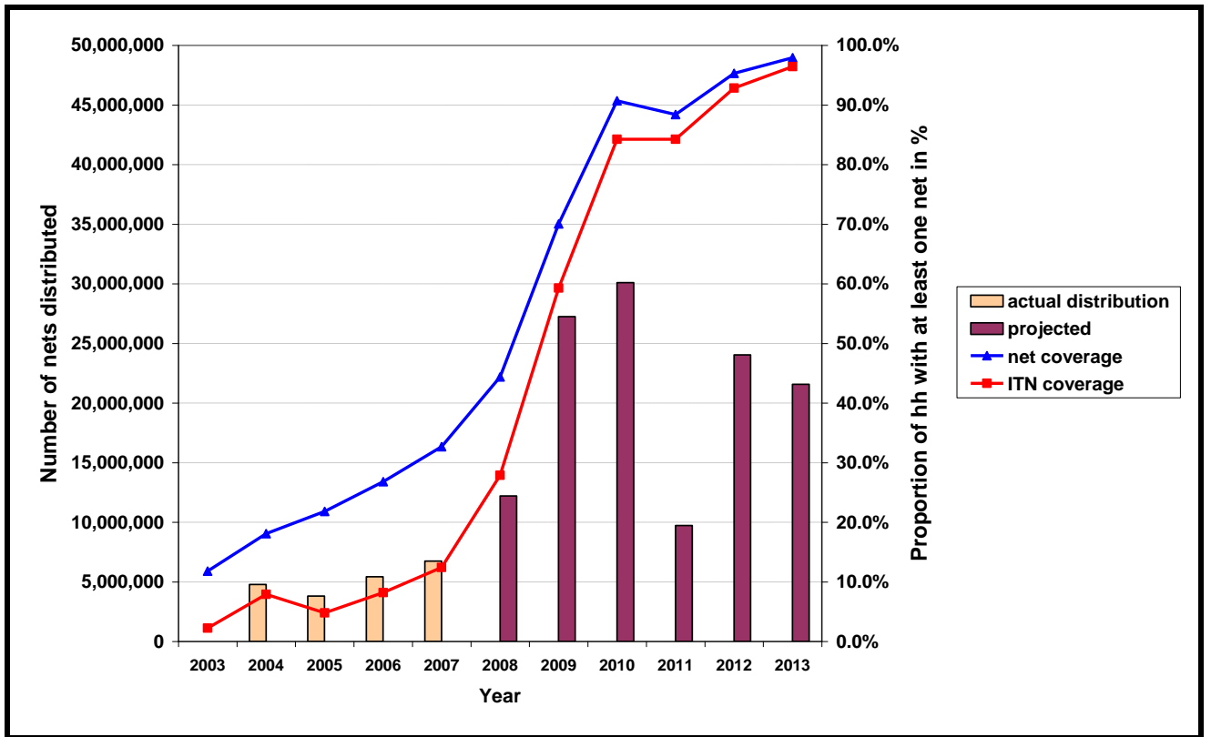
Figure 8: Estimated ITN coverage based on projected distributions
