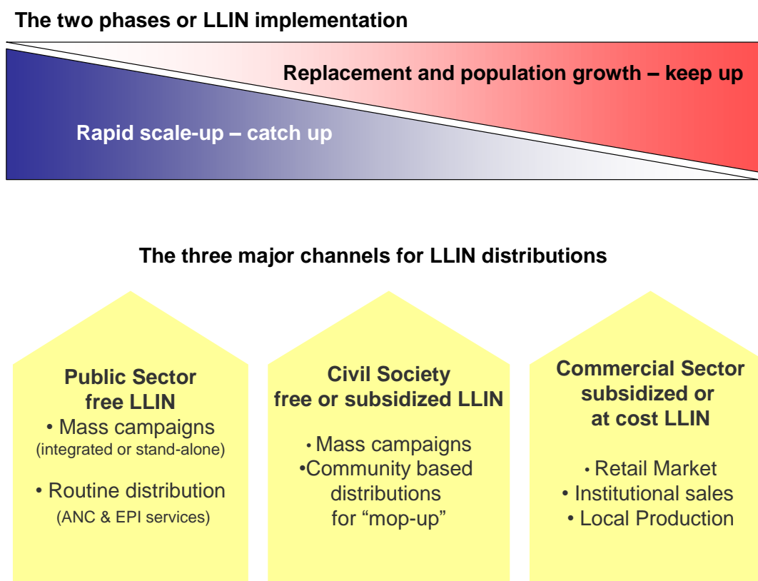
Figure 7: The mixed model of LLIN distribution
